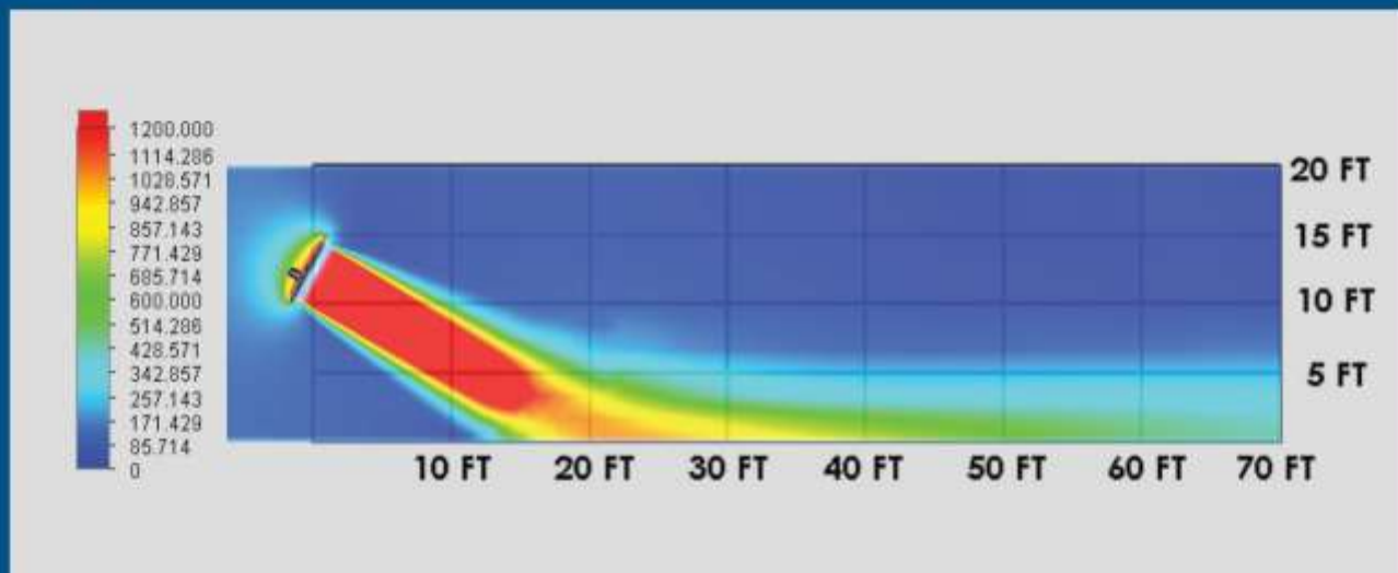
Figure 1 - Pattern of wind speed (ft / min) of the Blo-Air 52
